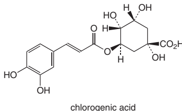
chlorogenic acid
