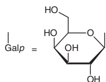
β-D-galactopyranosyl
